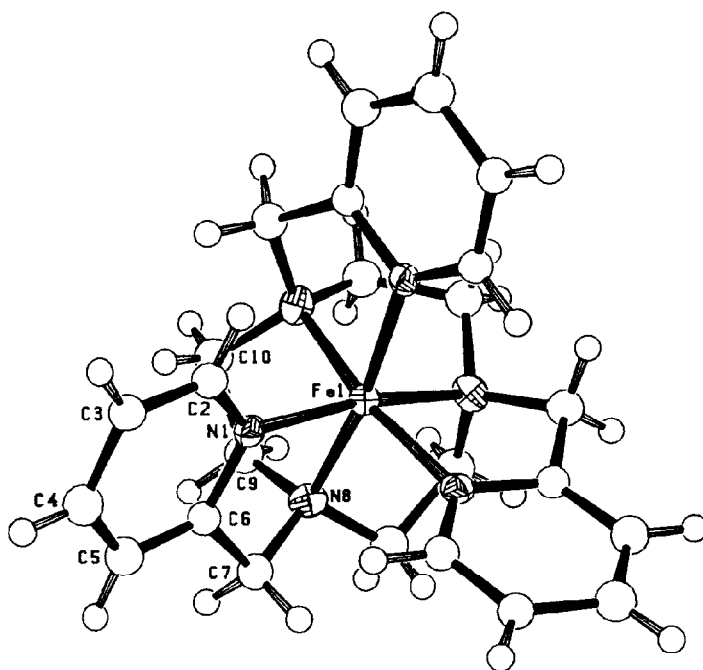
Fig. 12. ORTEP drawing of the molecular structure of one of the three crystallographically inequivalent cations in [\text{Fe}(\text{tptcn})](\text{ClO}_4)_2 [23].
