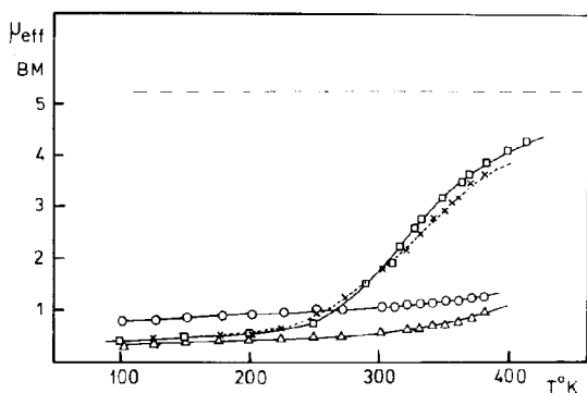
Fig. 3. Magnetic moment as a function of temperature for a series of [\text{Fe}(\text{tpen})]\text{X}_2 salts [16]: \square , X = perchlorate; \times , X = perchlorate, diluted into a zinc(II) host, \Delta , X = hexafluorophosphate; \circ , X = tetraphenyl borate.
