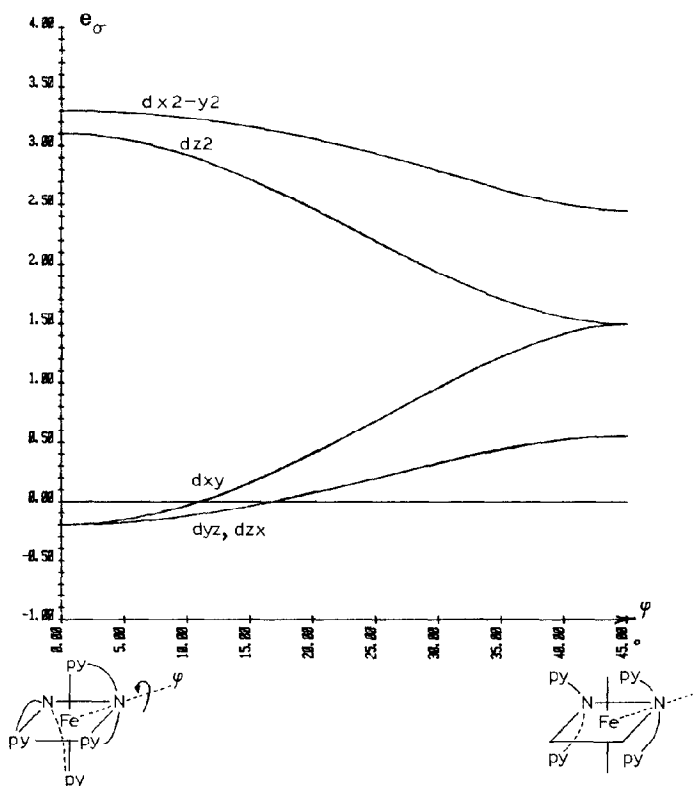
Fig. 23. AOM orbital energies (in units of e_\sigma ) as a function of the twist angle \phi for [\text{Fe}(\text{tpen})]^{2+} [17].
