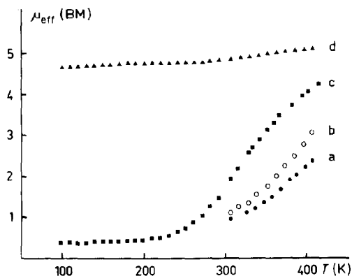
Fig. 4. Temperature dependence of the effective magnetic moments \mu_{\text{eff}} [13]: (a) [\text{Fe}(\text{tppn})](\text{ClO}_4)_2 \cdot \text{H}_2\text{O} , (b) [\text{Fe}(\text{tpchxn})](\text{ClO}_4)_2 \cdot 2 \text{H}_2\text{O} , (c) [\text{Fe}(\text{tpen})](\text{ClO}_4)_2 \cdot \text{H}_2\text{O} , (d) [\text{Fe}(\text{ltpen})](\text{ClO}_4)_2 \cdot \text{H}_2\text{O} .
