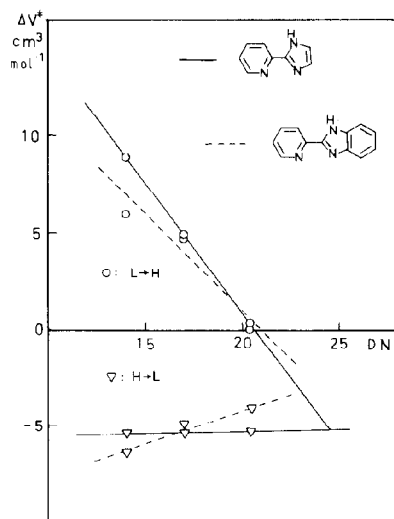
Fig. 20. Variation in the volume of activation as a function of the donor number of the solvent for two spin-equilibria systems: ○, low to high; ▽, high to low; —, [\text{Fe}(\text{pyim})_3](\text{ClO}_4)_2 ; ---, [\text{Fe}(\text{pyben})_3](\text{ClO}_4)_2 [65].
