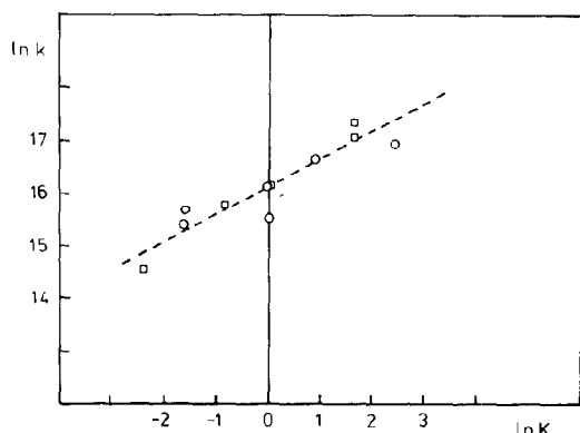
Fig. 19. Free-energy correlation for a series of spin-change reactions: ○, for k_{15} ; □, for k_{51} [18].
