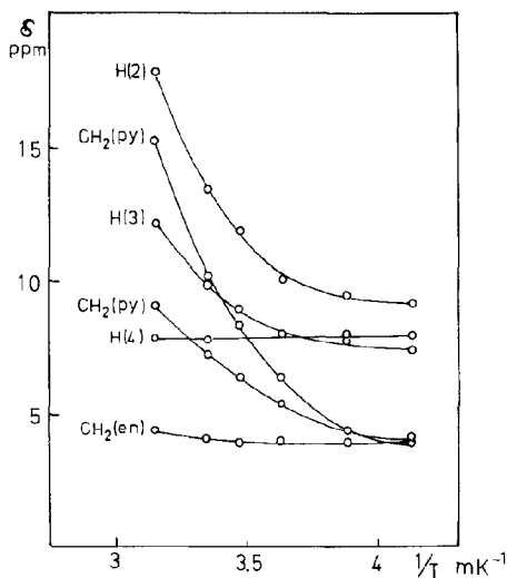
Fig. 24. Temperature variation of the ^1\text{H} NMR chemical shifts for [\text{Fe}(\text{tpen})]\text{I}_2 in a water-methanol (1:1 v/v) mixture [16].
